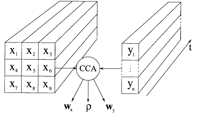
FIG. 1. Canonical correlation analysis between a 3 \times 3 region in the fMRI image and a set of n basis-functions.
