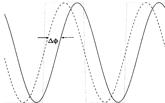
FIG. 5. The difference in phase between the fundamental frequency of Y(t) (solid) and the fundamental frequency of the paradigm (dashed) can be transformed into a time delay of the hemodynamic response. The dotted signal is the square-wave paradigm.
