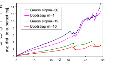
Fig. 3: Average distance to superset trajectory.
