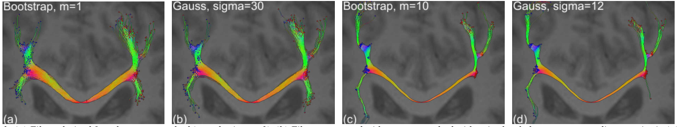
Fig. 1: (a) Fibers derived from bootstrap method (sample size m=1 ). (b) Fibers generated with our new method with noise level chosen corresponding to noise in (a). (c) Bootstrap, m=10 (d) Gauss, noise corresponding to (c). For better orientation the axial slice intersecting most of the fibers of a T1-weighted data set is shown.
