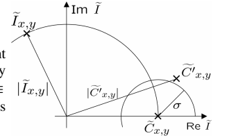
Fig. 2: Complex Gaussian noise.
